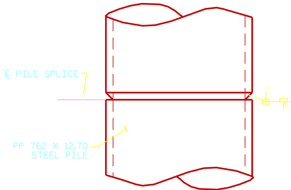
PIPE PILE SPLICE DETAIL
